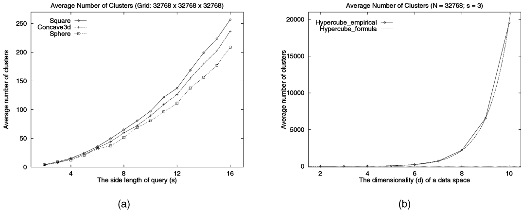
Fig. 12. Average number of clusters for higher-dimensional queries: (a) 3-dimensional queries and (b) d -dimensional hypercubic queries.
