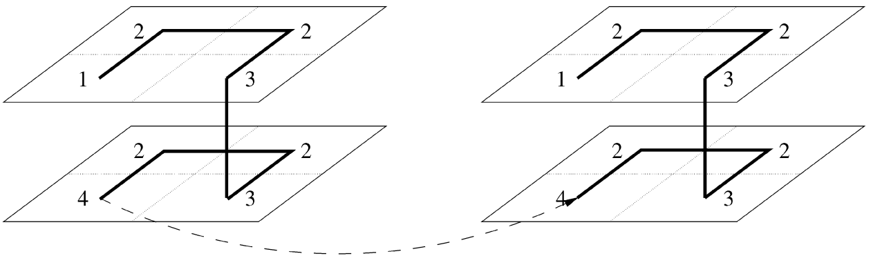
Fig. 5. The 4-dimensional Hilbert curve ( \mathcal{H}_k^4 with vertices representing \mathcal{H}_{k-1}^4 approximations annotated by their orientations.)
