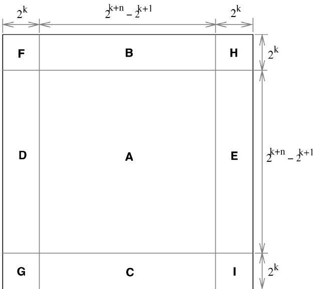
Fig. 7. \mathcal{H}_{k+n}^2 divided into nine subregions.
