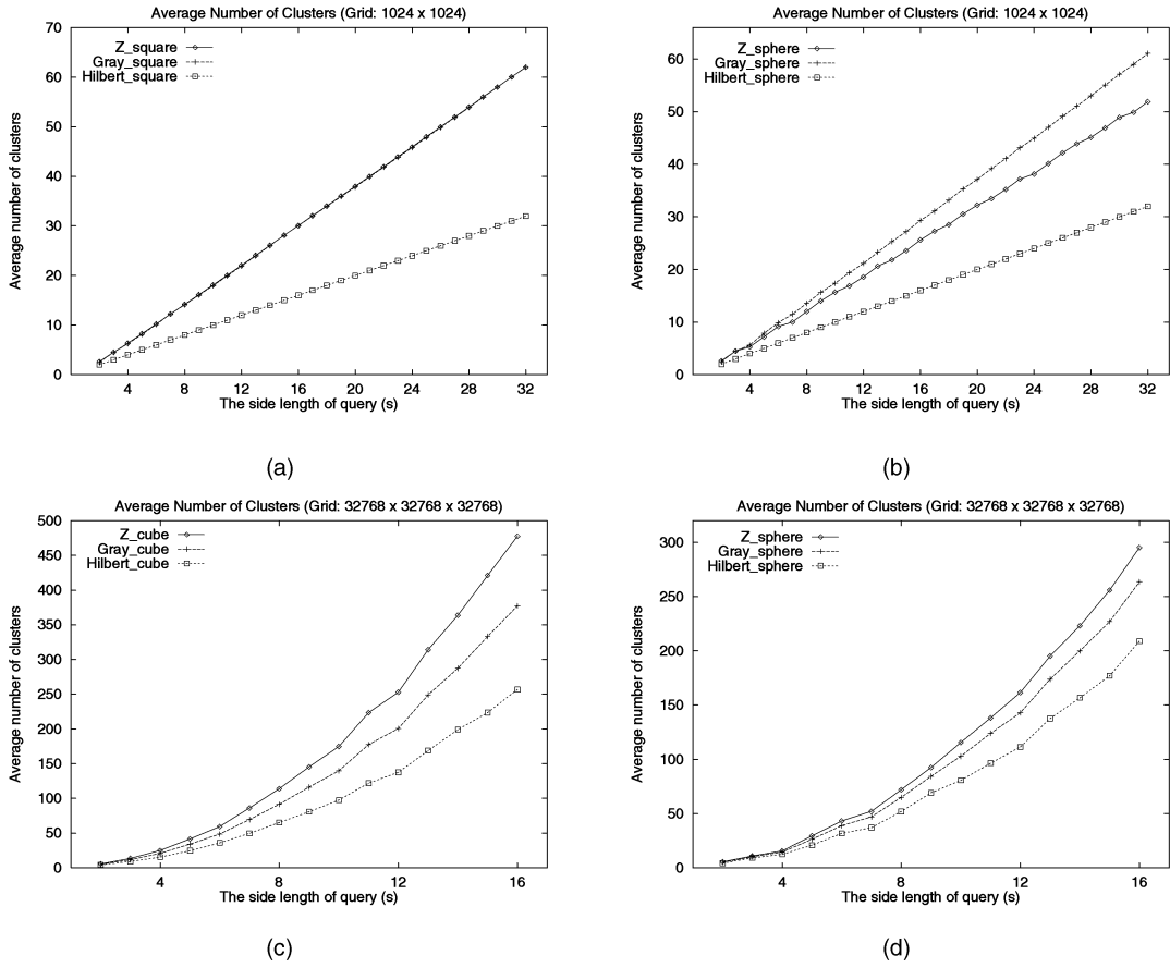
Fig. 14. Average number of clusters for three different space-filling curves: (a) 2-dimensional square queries, (b) 2-dimensional circular queries, (c) 3-dimensional cubic queries, and (d) 3-dimensional spherical queries.
