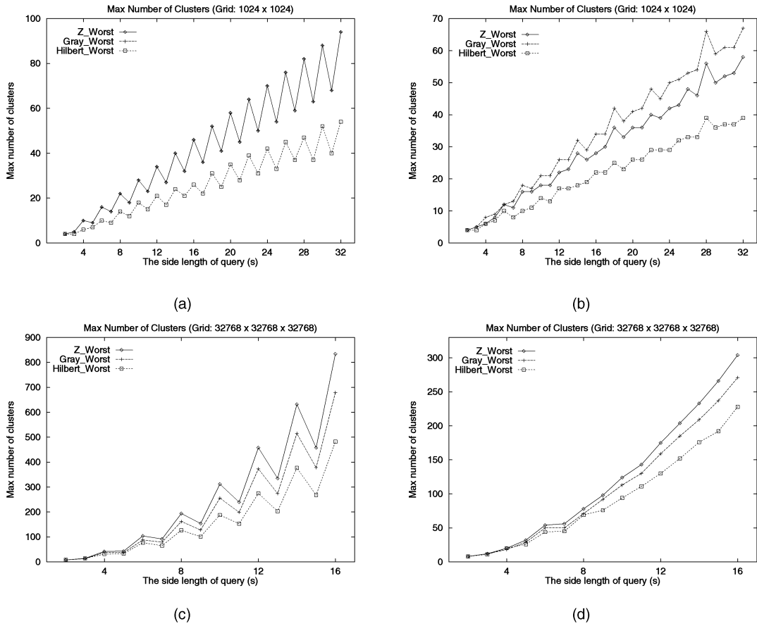
Fig. 13. Worst-case number of clusters for three different space-filling curves: (a) 2-dimensional square queries, (b) 2-dimensional circular queries, (c) 3-dimensional cubic queries, and (d) 3-dimensional spherical queries.
