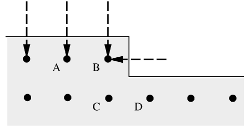
Fig. 6. Illustration of grid points facing surfaces.
